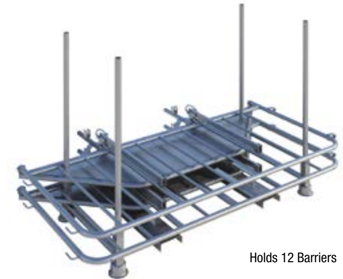
Police Barrier Collapsible Stillage Code: 02055245 Weight: 28kg Finish: Post Galvanised
