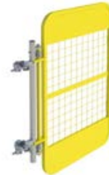
Ladder Access Gate (Spring Return) Code: 27051931 Weight: 11kg Finish: Electro Galvanised & Powder Coated
