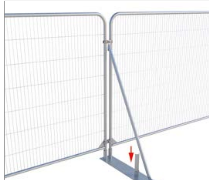
Fence Stabiliser c/w Large Plate - Euro Code F H Folding Stabiliser - Euro 095515383 F Ground Pin - Euro 0955931 Finish: Post Galvanised See page 36-37 for details of stabiliser components.
