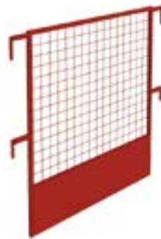
Smartguard End Panel Code: 27364031 Weight: 8.3kg Finish: Powder Coated
