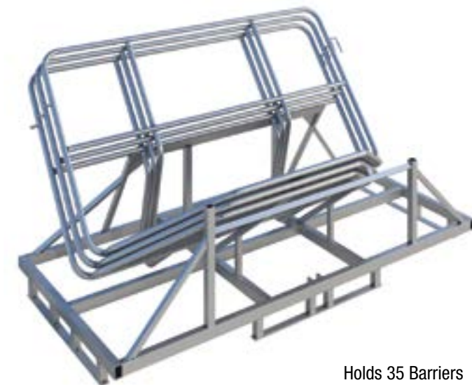
Police Barrier Stiff Stillage Code: 02055255 Weight: 100kg Finish: Post Galvanised
