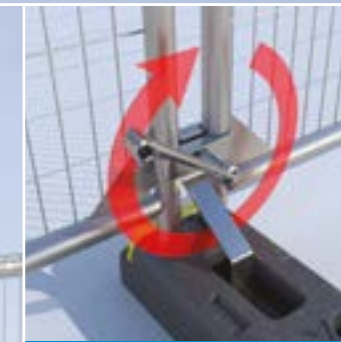
Assembly guides
